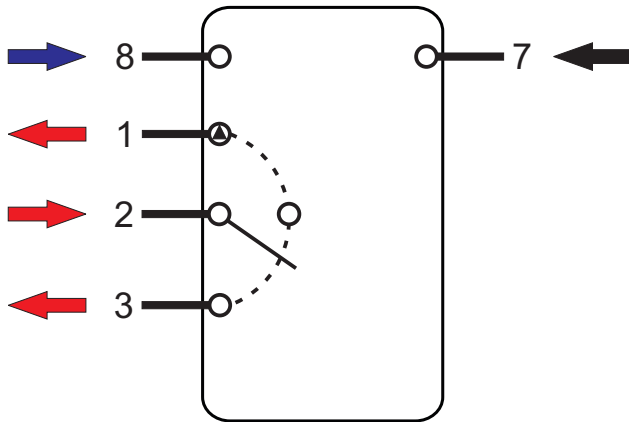
CIRCUIT DIAGRAM
